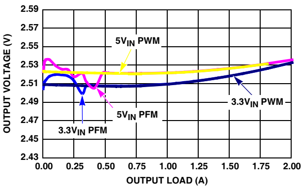
FIGURE 13. V_{\text{OUT}} REGULATION vs LOAD (1MHz, V_{\text{OUT}} = 2.5\text{V} )
