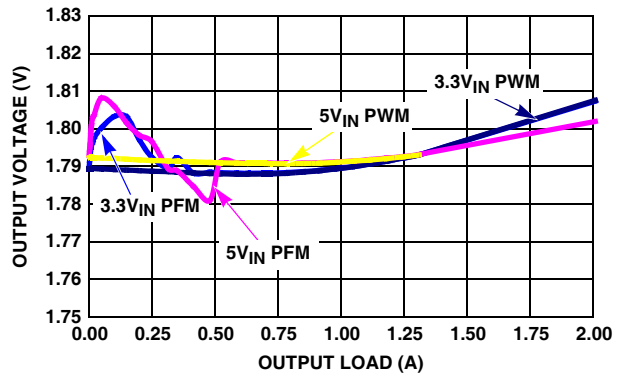
FIGURE 12. V_{\text{OUT}} REGULATION vs LOAD (1MHz, V_{\text{OUT}} = 1.8\text{V} )
