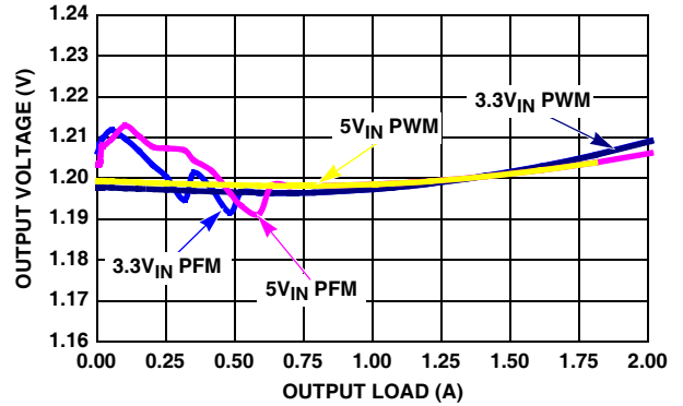
FIGURE 10. V_{\text{OUT}} REGULATION vs LOAD (1MHz, V_{\text{OUT}} = 1.2\text{V} )
