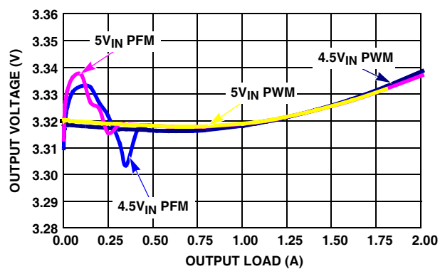
FIGURE 14. V_{\text{OUT}} REGULATION vs LOAD (1MHz, V_{\text{OUT}} = 3.3\text{V} )
