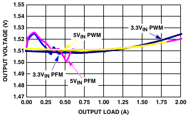
FIGURE 11. V_{\text{OUT}} REGULATION vs LOAD (1MHz, V_{\text{OUT}} = 1.5\text{V} )
